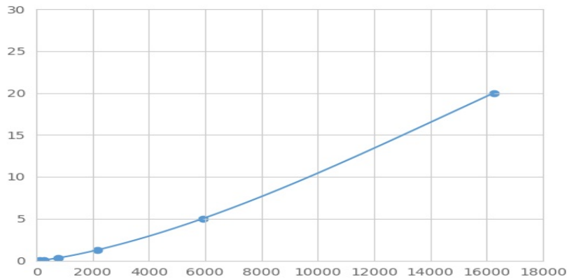
Typical Standard Curve for ASNS Magnetic Luminex Assay.
