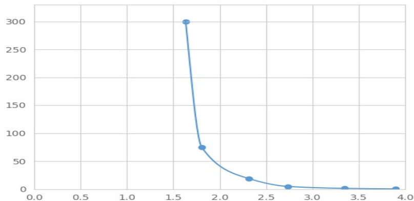
Typical Standard Curve for Dyn Magnetic Luminex Assay.
