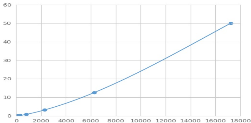
Typical Standard Curve for CA4 Magnetic Luminex Assay.
