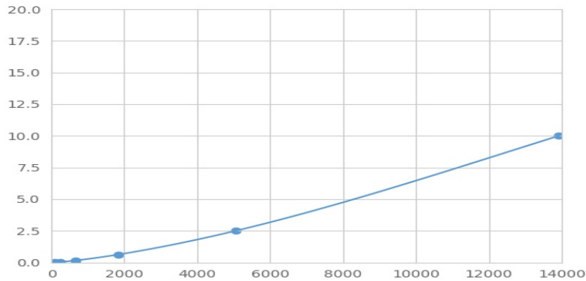
Typical Standard Curve for CAV1 Magnetic Luminex Assay.
