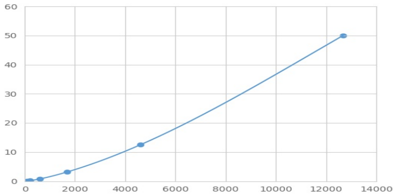
Typical Standard Curve for CHRNa5 Magnetic Luminex Assay.
