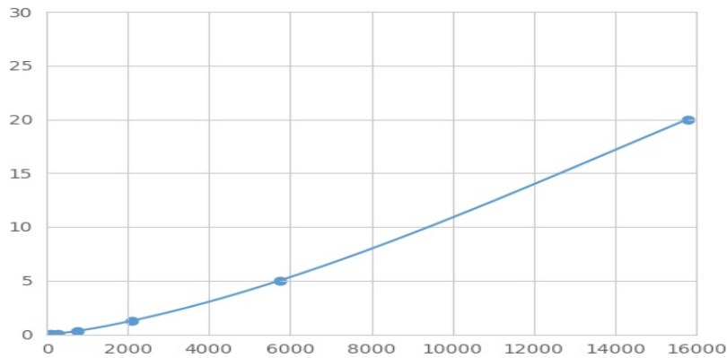
Typical Standard Curve for CLOCK Magnetic Luminex Assay.
