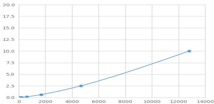
Typical Standard Curve for F5 Magnetic Luminex Assay.
