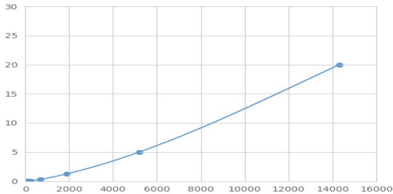
Typical Standard Curve for CLPS Magnetic Luminex Assay.
