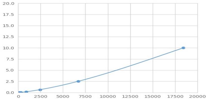
Typical Standard Curve for CPLX2 Magnetic Luminex Assay.
