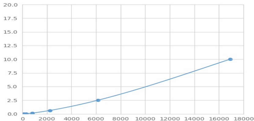
Typical Standard Curve for CDKN3 Magnetic Luminex Assay.
