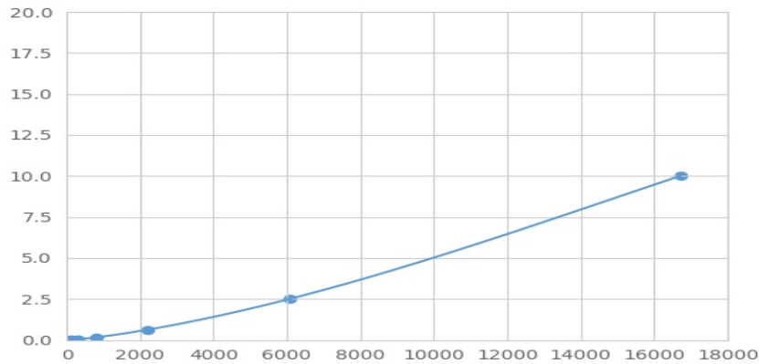
Typical Standard Curve for CST1 Magnetic Luminex Assay.
