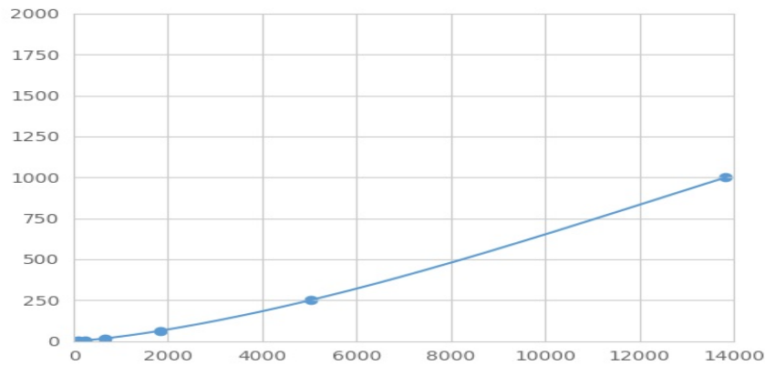
Typical Standard Curve for CK5 Magnetic Luminex Assay.
