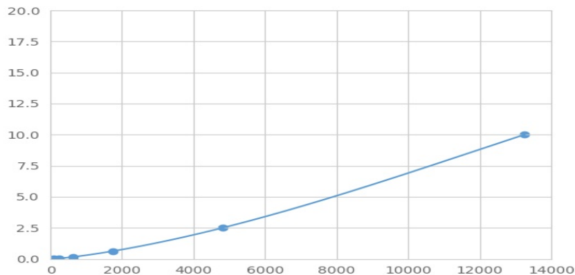
Typical Standard Curve for DAPK1 Magnetic Luminex Assay.
