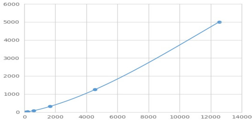
Typical Standard Curve for DPYSL2 Magnetic Luminex Assay.
