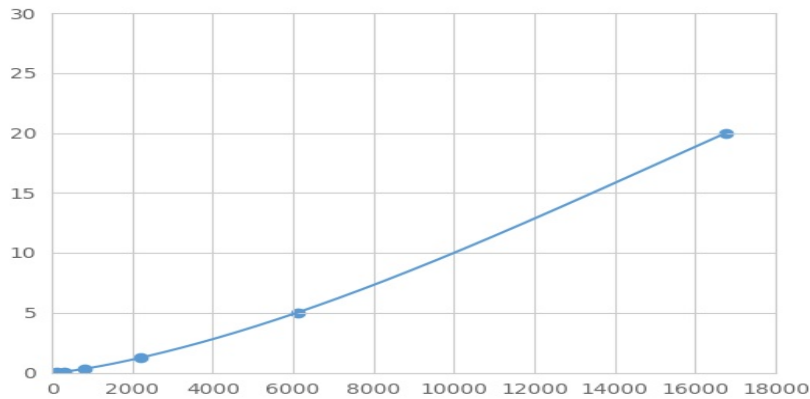
Typical Standard Curve for DLG4 Magnetic Luminex Assay.
