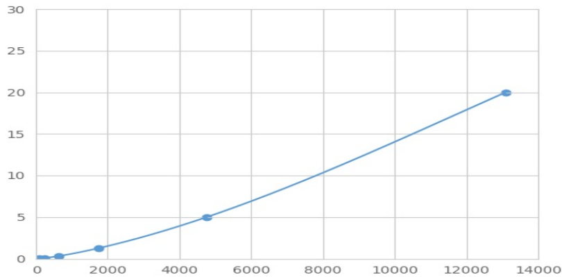
Typical Standard Curve for ESAM Magnetic Luminex Assay.
