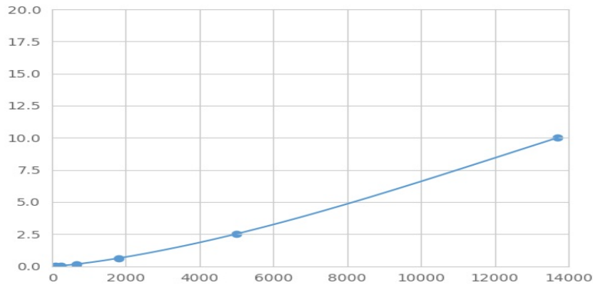
Typical Standard Curve for FKBPL Magnetic Luminex Assay.
