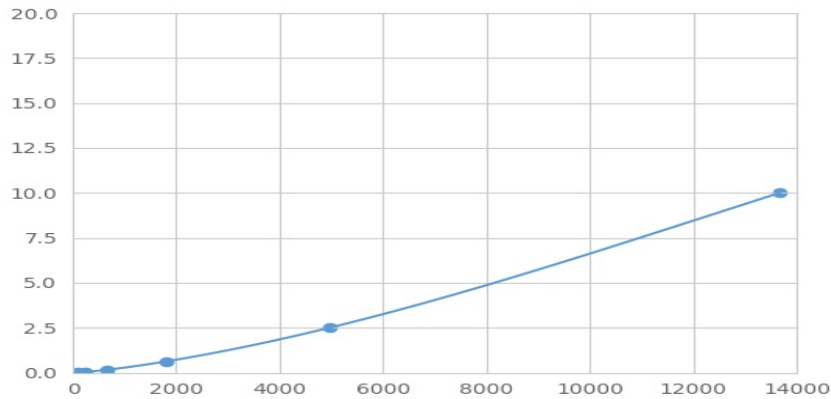
Typical Standard Curve for FASL Magnetic Luminex Assay.
