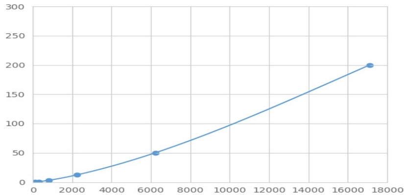
Typical Standard Curve for FTH Magnetic Luminex Assay.
