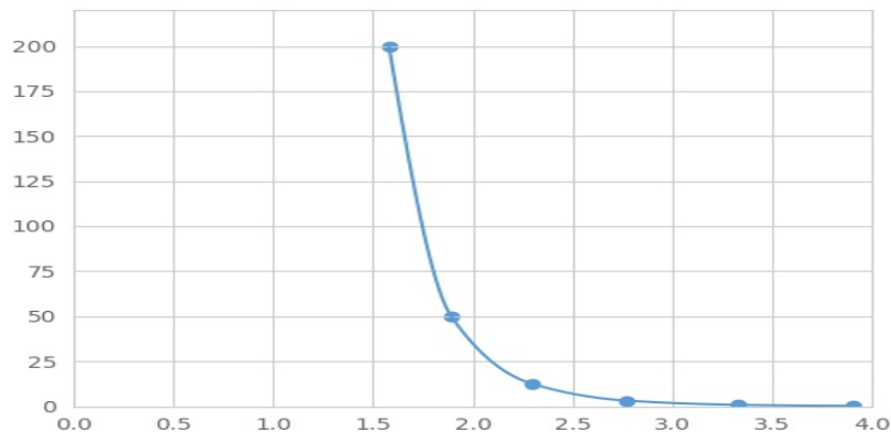
Typical Standard Curve for HBF Magnetic Luminex Assay.
