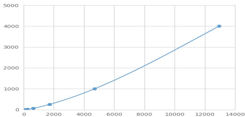
Typical Standard Curve for FDP Magnetic Luminex Assay.
