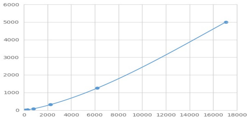
Typical Standard Curve for FCN3 Magnetic Luminex Assay.
