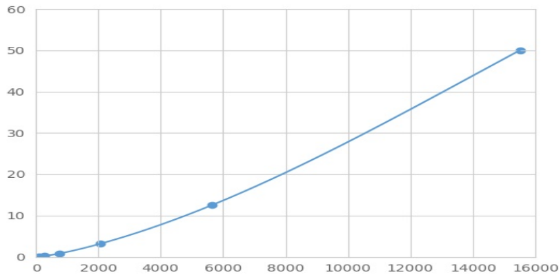
Typical Standard Curve for FLOT1 Magnetic Luminex Assay.
