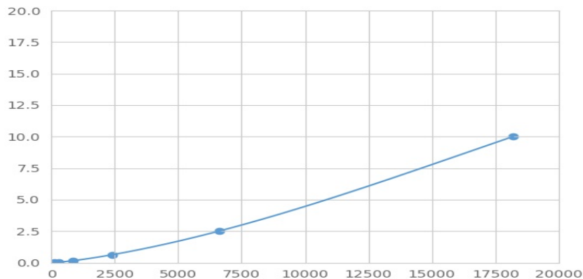
Typical Standard Curve for GNb1 Magnetic Luminex Assay.
