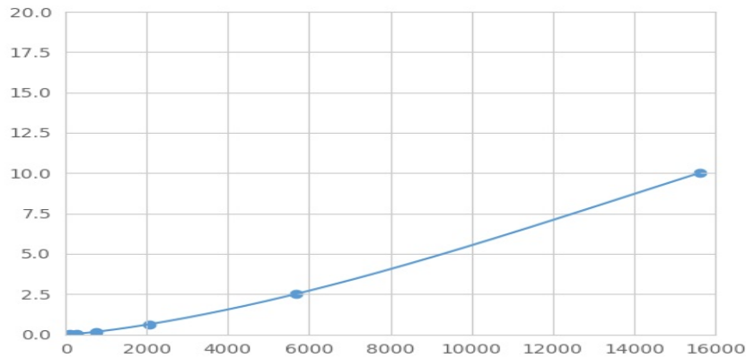
Typical Standard Curve for GPR37 Magnetic Luminex Assay.
