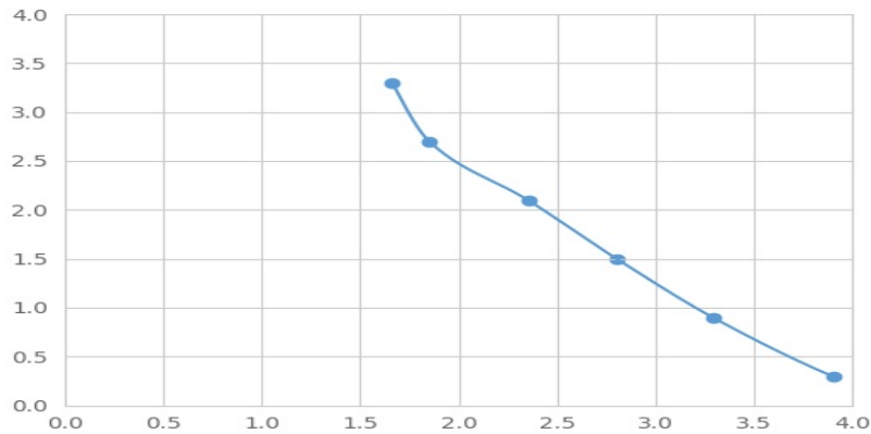
Typical Standard Curve for gABA Magnetic Luminex Assay.
