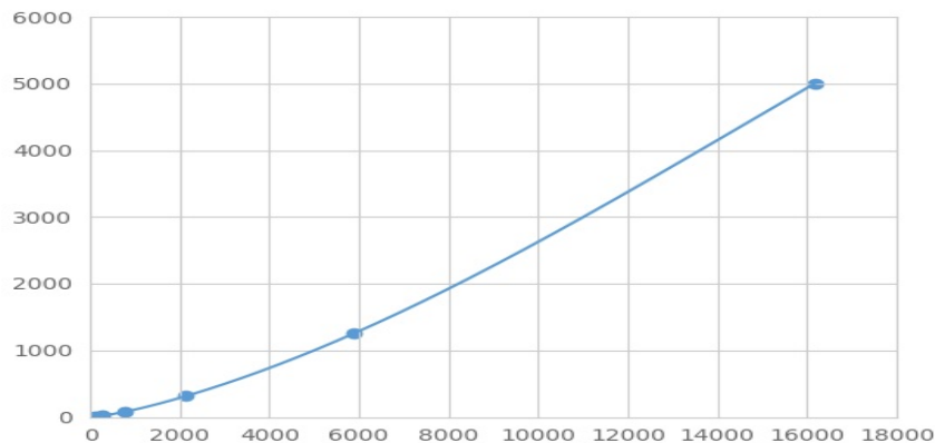
Typical Standard Curve for GSTa1 Magnetic Luminex Assay.
