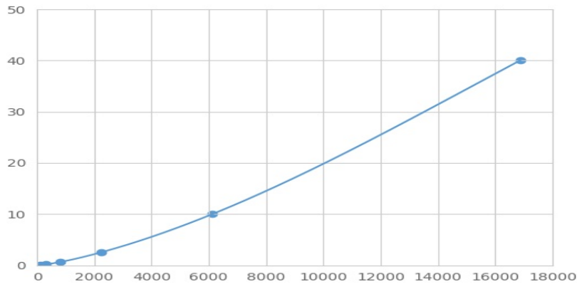
Typical Standard Curve for HSPb2 Magnetic Luminex Assay.
