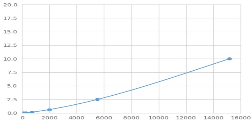
Typical Standard Curve for HS2ST1 Magnetic Luminex Assay.
