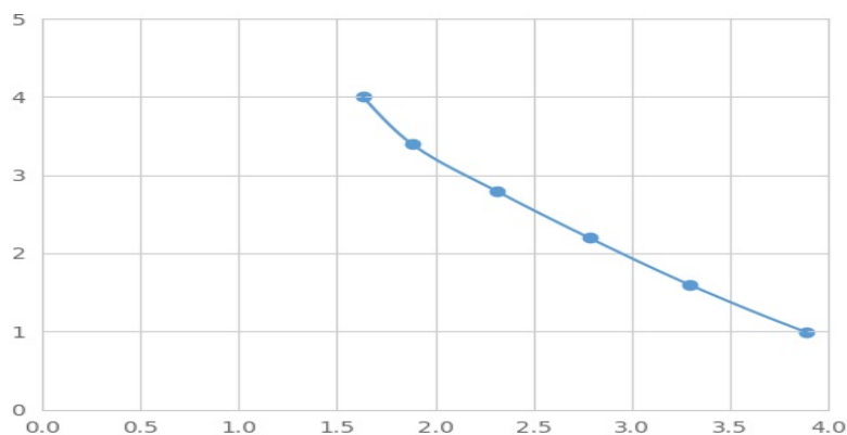
Typical Standard Curve for KLK14 Magnetic Luminescence Assay.
