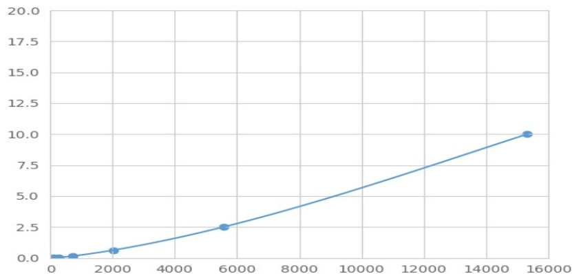
Typical Standard Curve for LRP6 Magnetic Luminex Assay.
