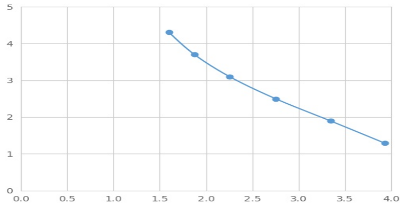
Typical Standard Curve for LHb Magnetic Luminex Assay.
