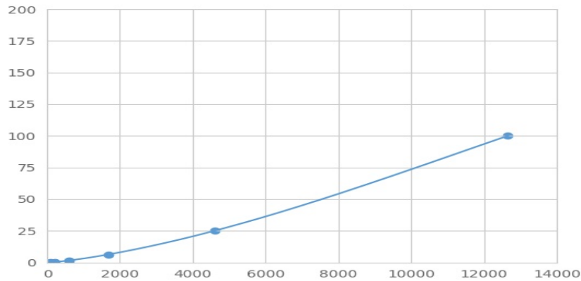
Typical Standard Curve for MAPK14 Magnetic Luminex Assay.
