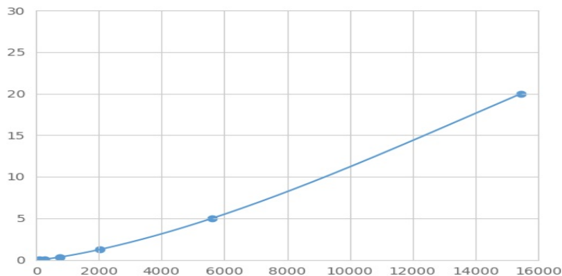
Typical Standard Curve for NPR3 Magnetic Luminex Assay.
