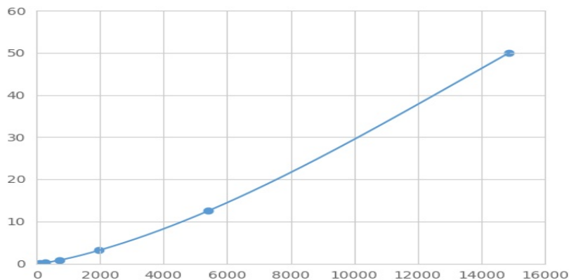
Typical Standard Curve for ORM2 Magnetic Luminex Assay.
