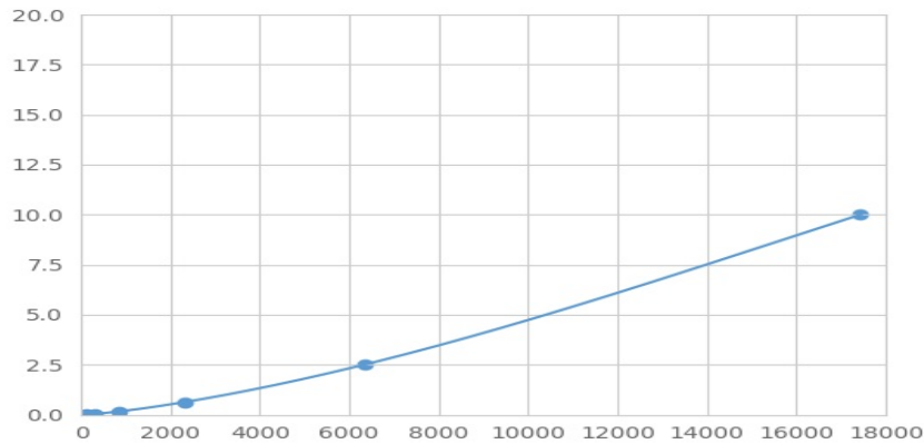
Typical Standard Curve for PPARa Magnetic Luminex Assay.
