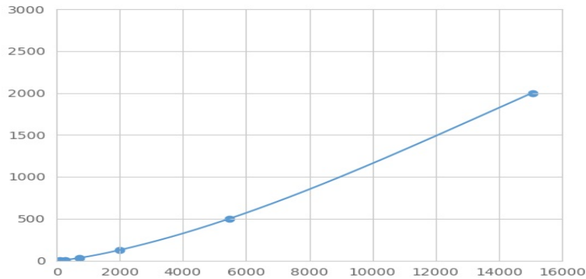
Typical Standard Curve for GP1BB Magnetic Luminex Assay.
