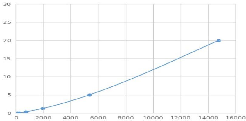
Typical Standard Curve for POLg1 Magnetic Luminex Assay.
