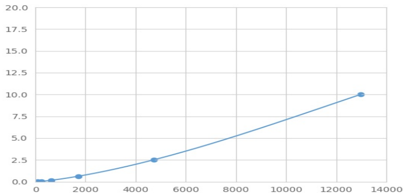
Typical Standard Curve for PS2 Magnetic Luminex Assay.
