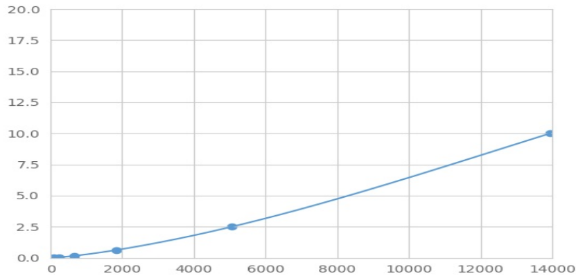
Typical Standard Curve for PSMB9 Magnetic Luminex Assay.
