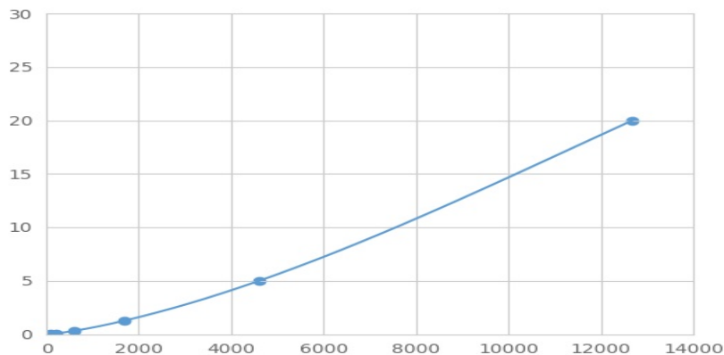
Typical Standard Curve for PDI Magnetic Luminex Assay.
