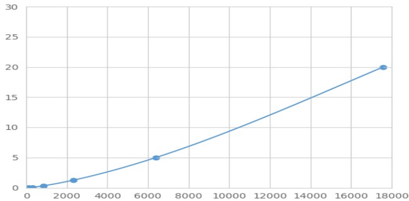
Typical Standard Curve for PKCa Magnetic Luminex Assay.
