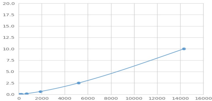
Typical Standard Curve for RXFP3 Magnetic Luminex Assay.
