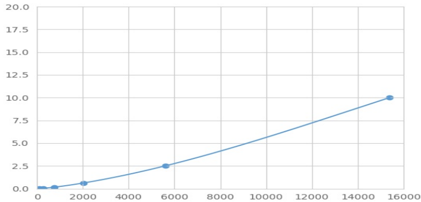
Typical Standard Curve for RBP3 Magnetic Luminex Assay.
