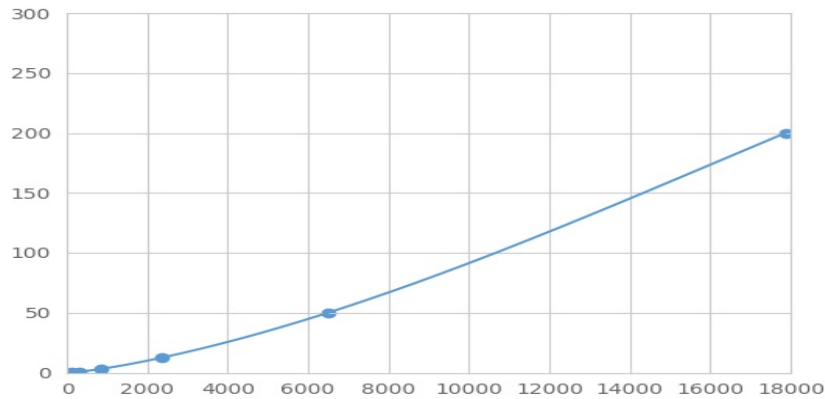
Typical Standard Curve for S100B Magnetic Luminex Assay.
