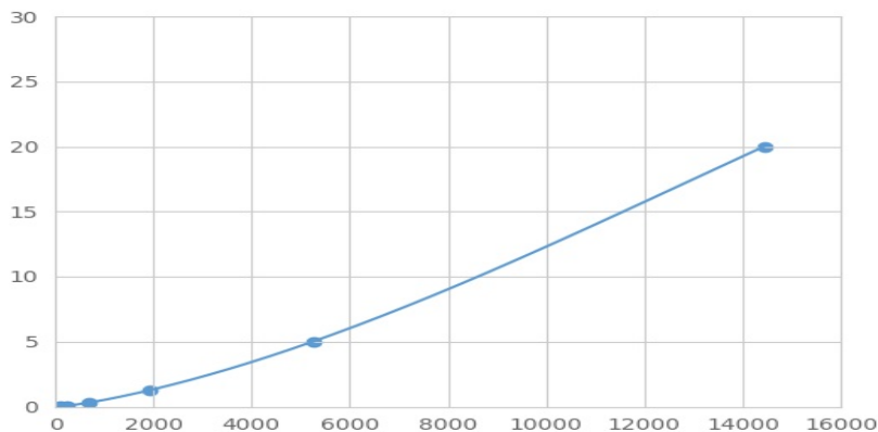
Typical Standard Curve for SCG2 Magnetic Luminex Assay.
