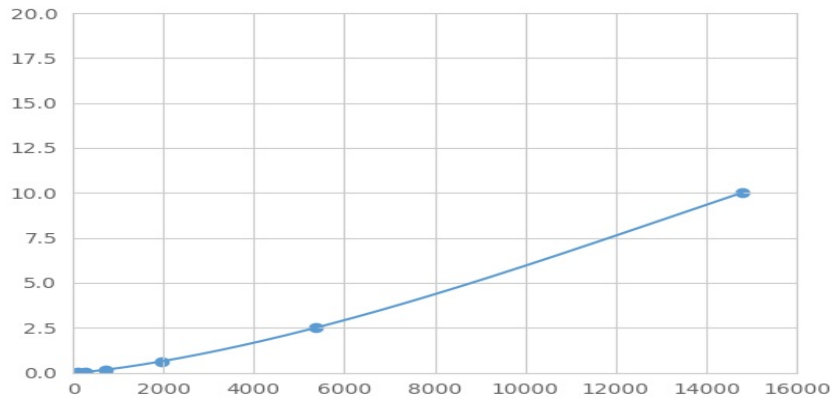
Typical Standard Curve for SRY Magnetic Luminex Assay.
