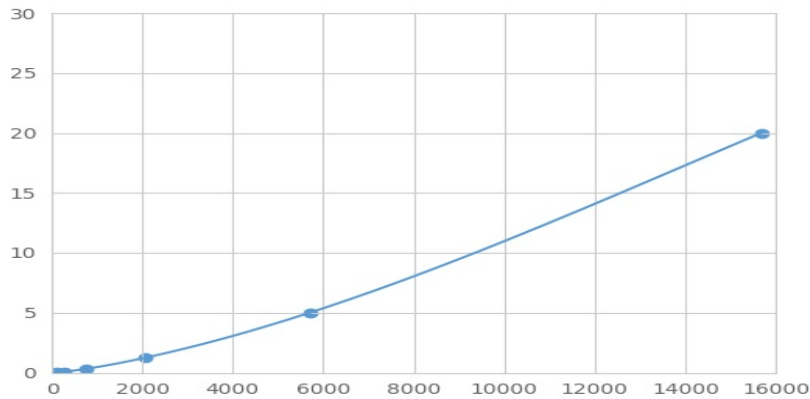
Typical Standard Curve for SLC30A5 Magnetic Luminex Assay.
