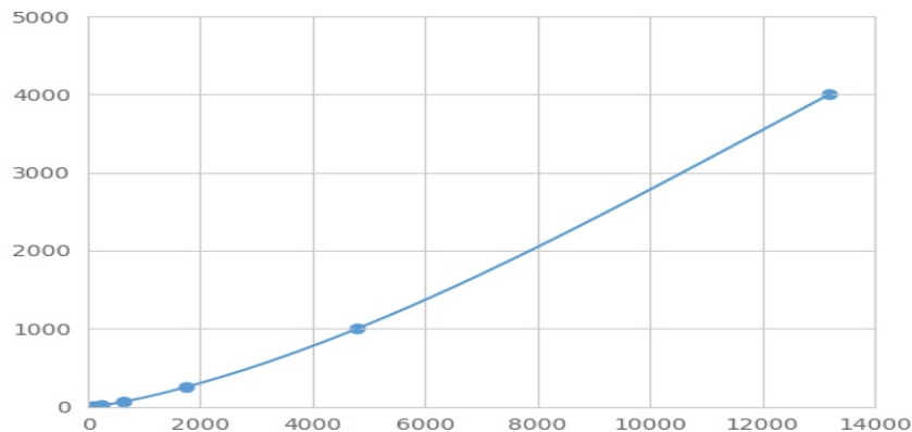
Typical Standard Curve for TDP43 Magnetic Luminex Assay.
