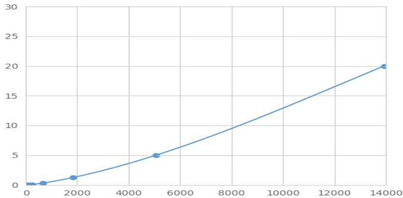
Typical Standard Curve for TGFbR2 Magnetic Luminex Assay.
